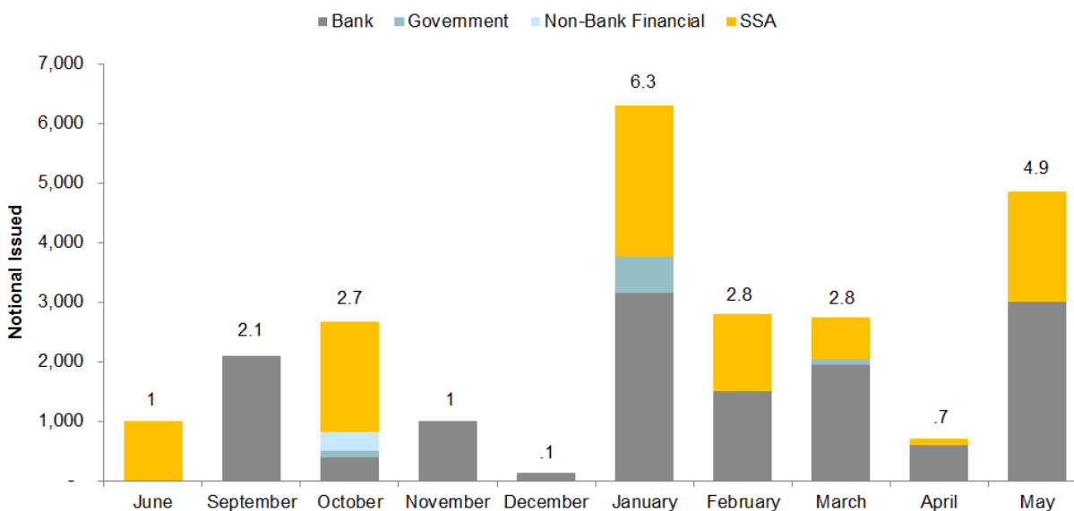
Figure 6: SONIA Issuance
