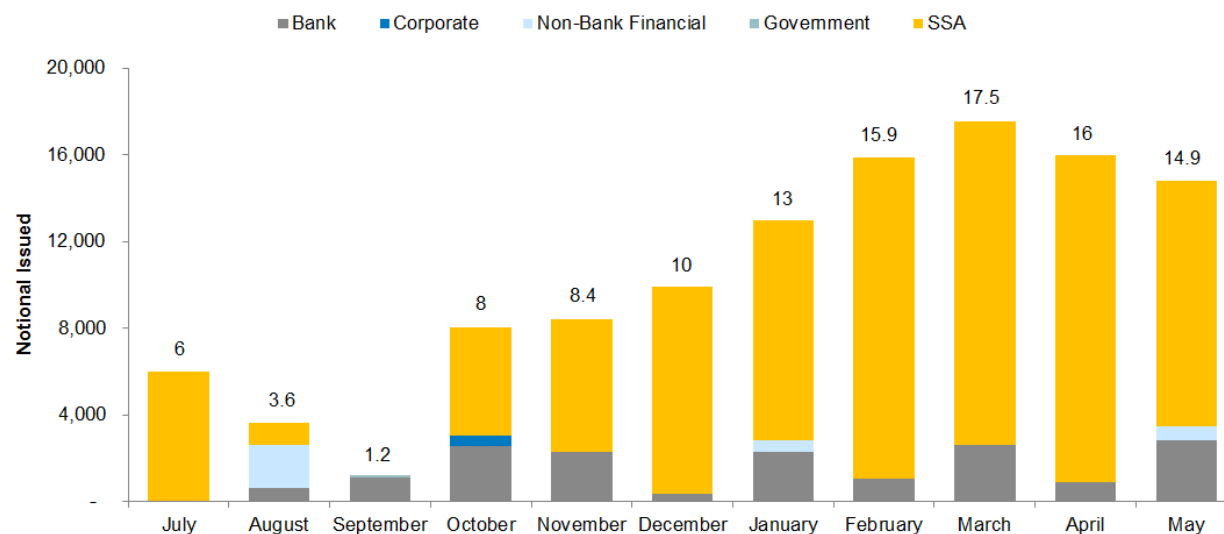
Figure 5: SOFR Issuance
